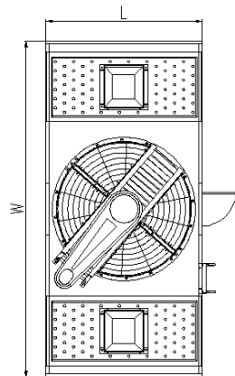
PLAN VIEW
