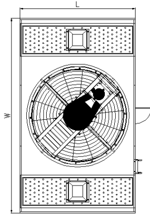
PLAN VIEW
