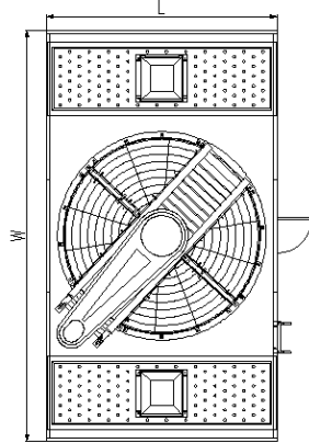
PLAN VIEW
