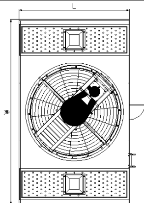
PLAN VIEW
