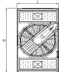
PLAN VIEW
