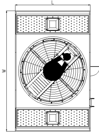
PLAN VIEW
